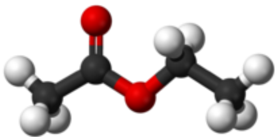
Fig 1- Ethyle acetate chemical structure
