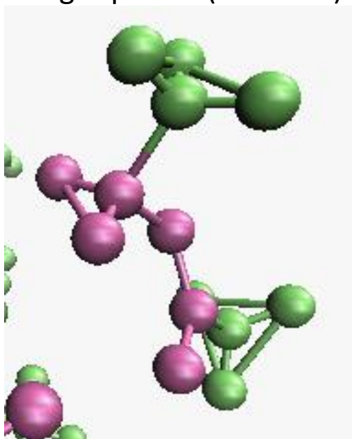
Fig 3- Ethyle acetate from the Lammps-trajectory file using VMD
