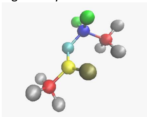
Fig 2- Ethyle acetate produced from moltemplate and plotted using topotool ( on VMD)
