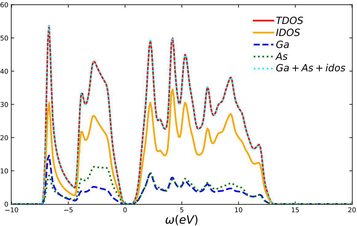
GaAs without SOC
