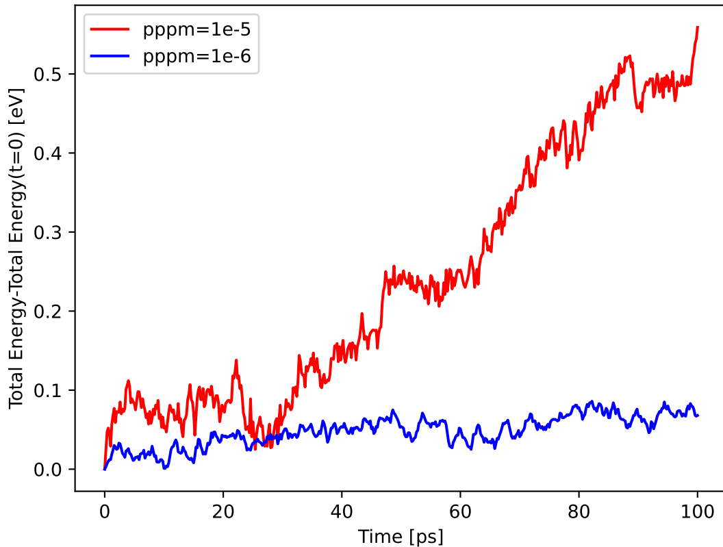
Graphene/water PPPM compare, dt=0.2 fs
