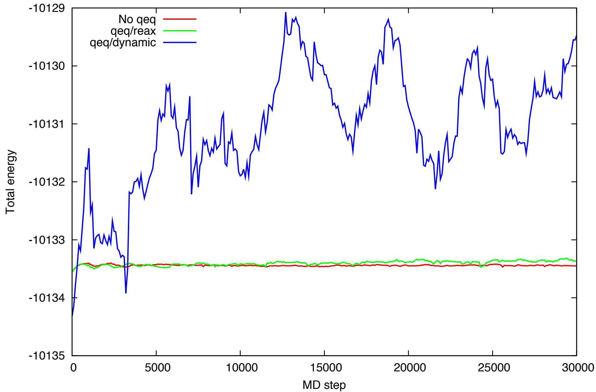
ReaxFF example
